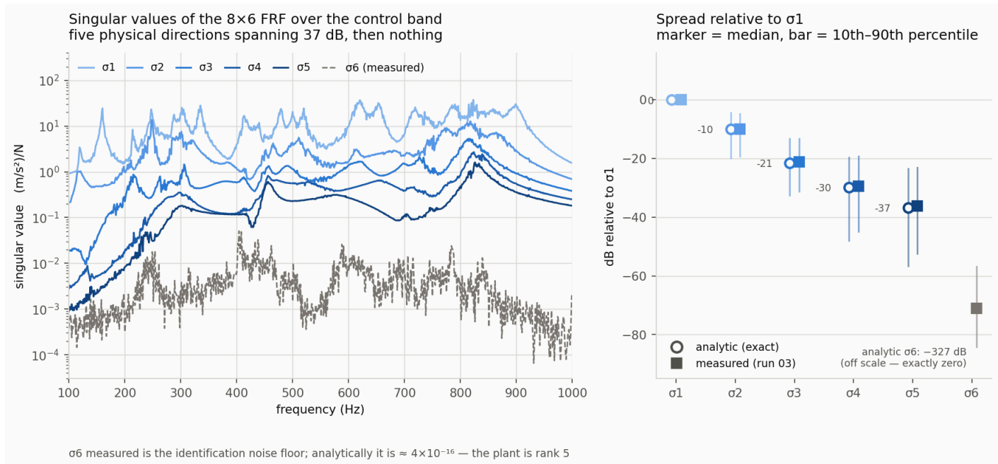
Singular values of the 8×6 FRF over the control band. Left: the measured in-control FRF, the matrix every law actually inverts. Right: median and 10th–90th percentile of each singular value relative to \sigma_1 , analytic against measured.
